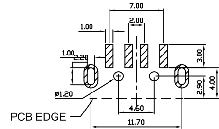
SUGGESTED PCB LAYOUT TOP VIEW
