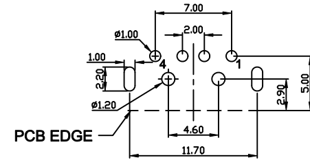
SUGGESTED PCB LAYOUT TOP VIEW
