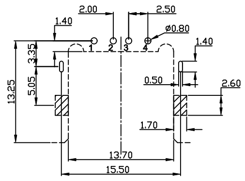
RECOMMEND PCB LAYOUT TOP VIEW
