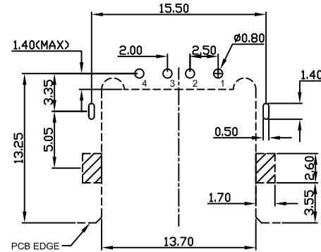
RECOMMEND PCB LAYOUT TOP VIEW
